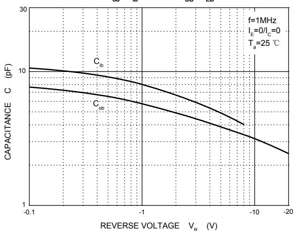
C_{ob}/C_{ib} — V_R/V_{EB}
