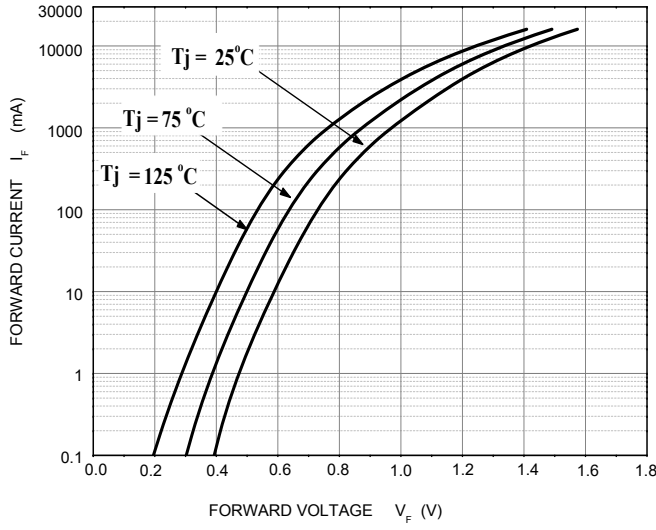
Forward Characteristics
