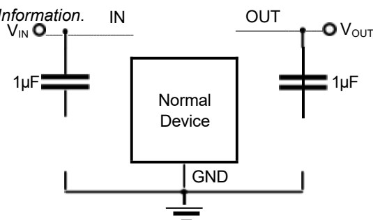
Typical Application Circuits
